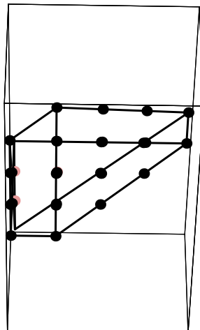
FIGURE 3. Twisted cube projected into \mathfrak{t}^*
